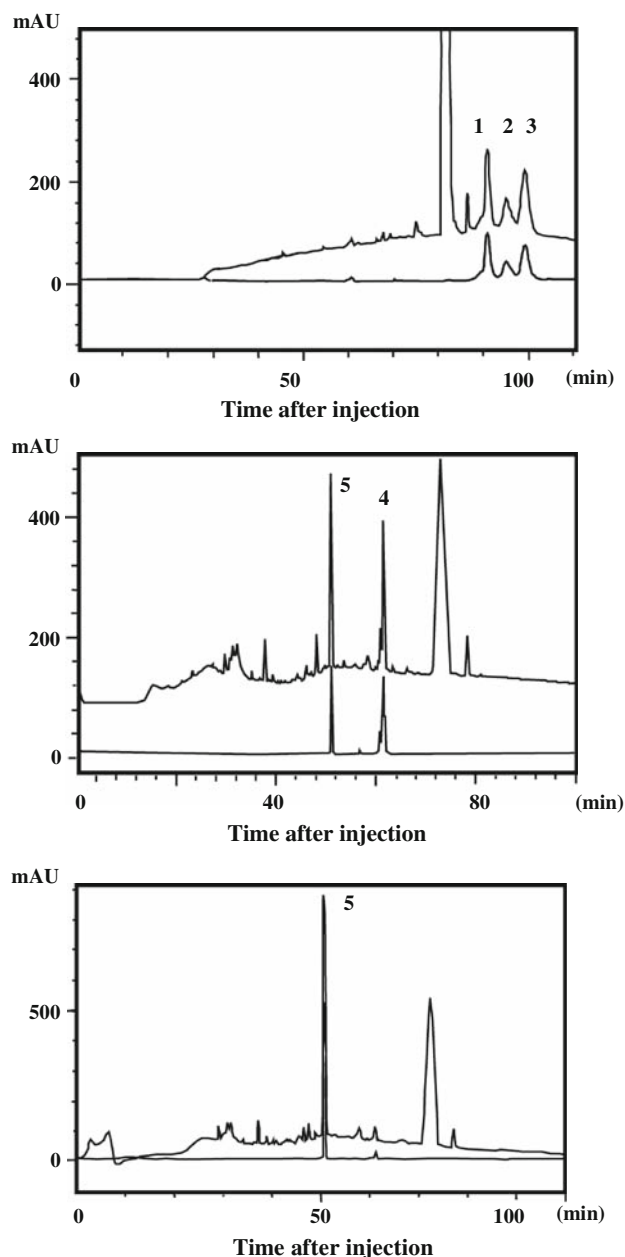
Fig. 4 Elution profiles of nontreated ( top ), 30-min-lipase-treated ( middle ) and 180-min-lipase-treated ( bottom ) purified B. clarkii K24-1U cytochromes c -550 in presence of 0.1% Triton X-100 as determined by reverse-phase HPLC with a column. The upper and lower elution patterns in each elution profile indicate monitoring at 214 and 406 nm, respectively. The molecular masses determined by MALDI-TOF MS were as follows: peak 1 11,082 Da, peak 2 11,097 Da, peak 3 11,111 Da, peak 4 10,857 Da, peak 5 10,632 Da
