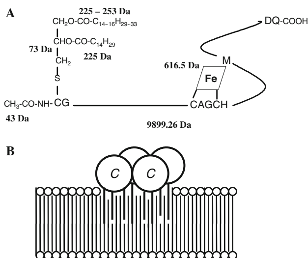
Fig. 5 Model of predicted structure of mature processed cytochrome c -550. a Model of posttranscriptional modification. The numbers indicate the molecular masses of the respective portions. b Model of tetrameric structure binding to outer membrane surface. The upper side is the extracellular membrane and the lower side is the intracellular membrane. The round and membrane-binding moieties are the protein and anchor parts, respectively
