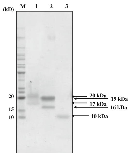
Fig. 1 SDS-PAGE of nontreated and lipase-treated cytochromes c -550 purified from B. clarkii K24-1U followed by CBB staining. Lane 1 nontreated cytochrome c -550, lane 2 intermediate state of lipase-treated (30 min) cytochrome c -550, lane 3 lipid-free cytochrome c -550 (lipase-treated: 180 min)
