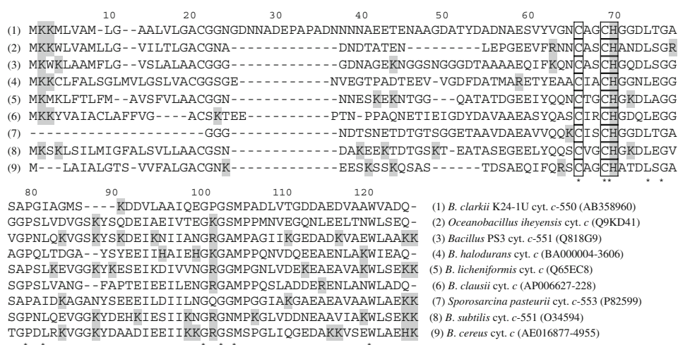
Fig. 3 Amino acid sequence alignment of cytochrome c -550 from Bacillus clarkii K24-1U and other diacylglycerol anchored cytochromes c from Gram-positive bacteria. Additional sequence of Gly 22 -Asn 34 (cytochrome c -550 numbering) was observed only in cytochrome c -550. The boxed sequences are heme-binding sites. Basic amino acids are highlighted in gray. Asterisks are identical amino acid residues
